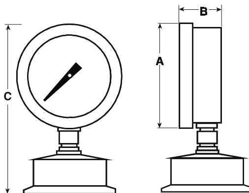
Lower-Connected (Vertical) Dimensions
