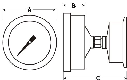
Back-Connected (Horizontal) Dimensions
