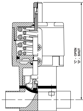
Spring Close EC Actuator With Limit travel stop
