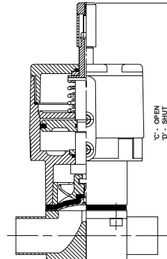
Spring Open EC Actuator With Limit travel stop
