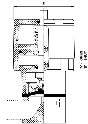
Spring Open EC Actuator
