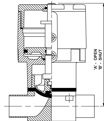
Double Acting EC Actuator
