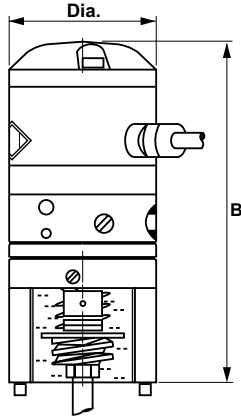
Mini electropneumatic positioner with feedback spring and position indicator
